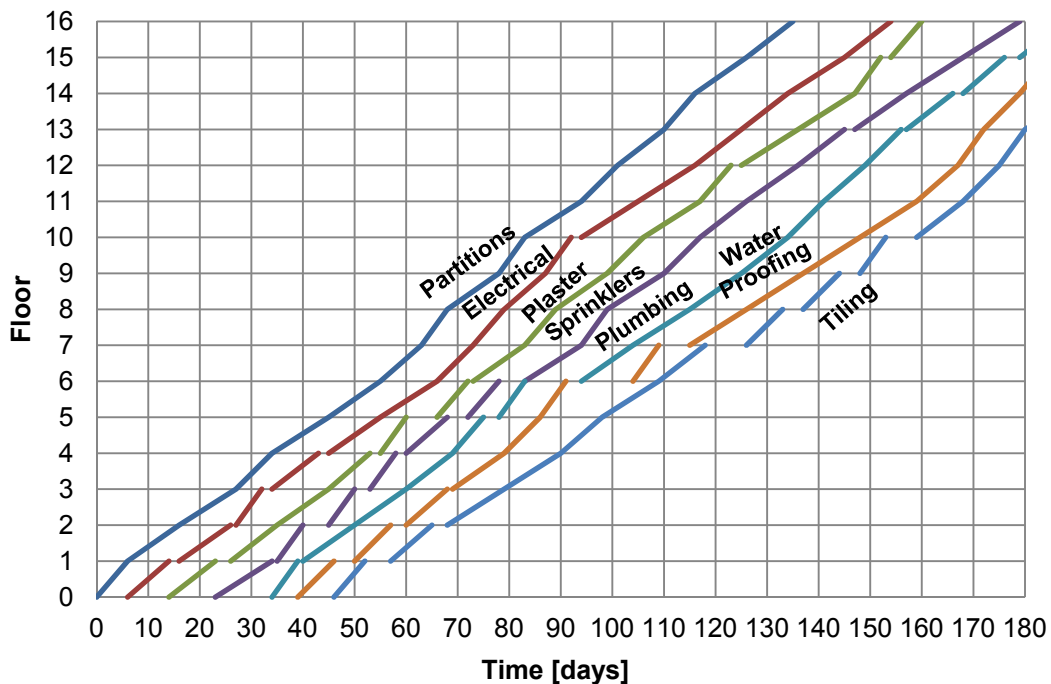
Figure 2: Example of flowline chart generated by simulation
