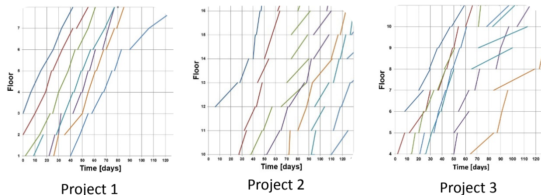
Figure 1: flowline charts of three real projects
