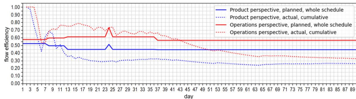
Figure 2: General flow efficiencies averaged over all work packages or takt areas.
